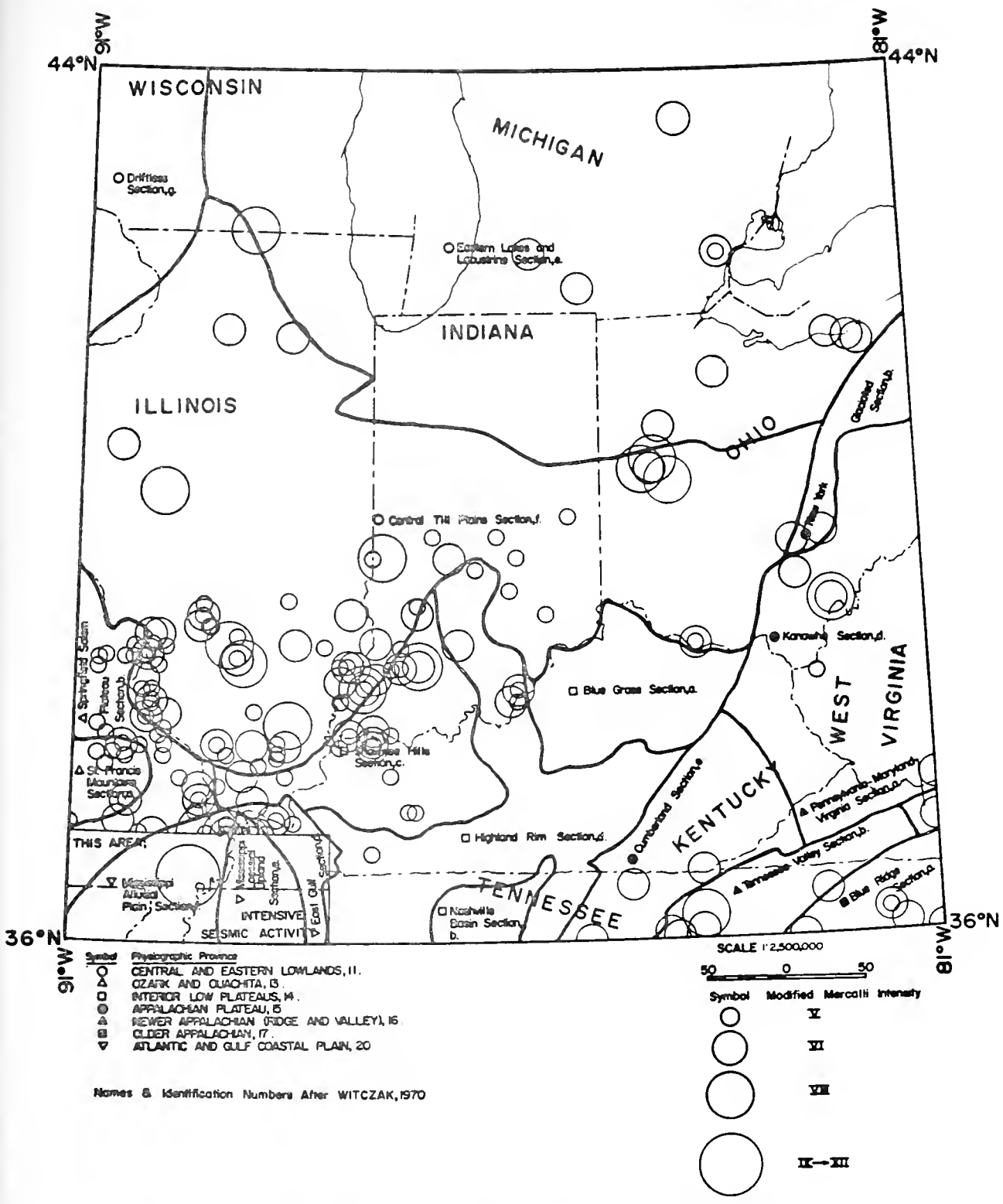
FIGURE 6 REGIONAL PHYSIOGRAPHY.
